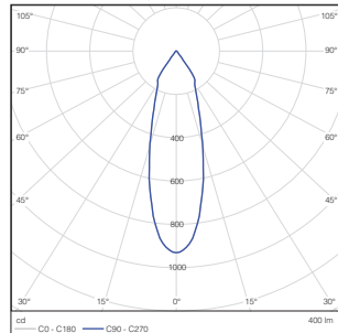
Spotlight Hydro COB IP65 Fire Rated 6W 10V 927
