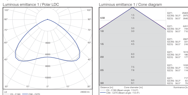
Highbay Pro-Clean (HACCP) 200W 4000K 90° 1-10V Dim. Grey
