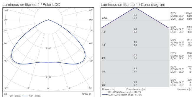
Highbay Pro-Clean (HACCP) 150W 4000K 90° 1-10V Dim. Grey
